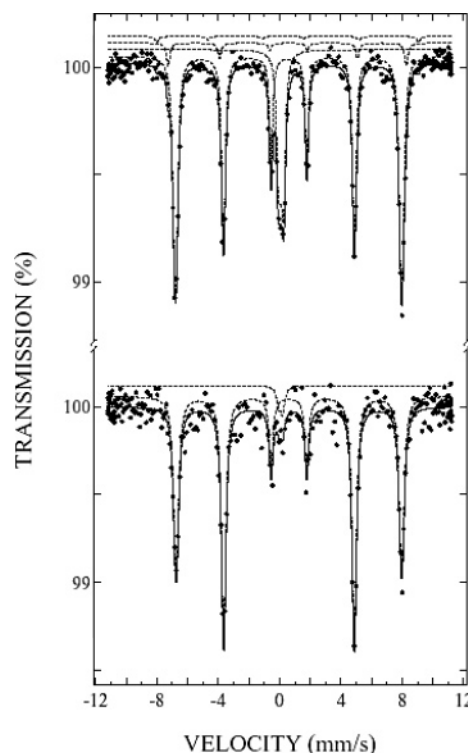
Figure 8. Mössbauer spectra for a \text{Sr}_2\text{FeMoO}_6 sample sintered at 1150 °C for 100 h recorded at (a) 77 K, 0 T and (b) 77 K, 600 mT. The upper spectrum exhibits the presence of superparamagnetism, which has been suppressed using an applied field in the lower spectrum. The average angle between the domain magnetization and direction of the beam was fitted to 79.7°. The components used in the fitting are displayed above each spectrum. Reading from the top they are AS, M2, SP, M1 and SP, M1 for the upper and lower spectrum, respectively.
