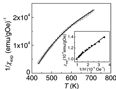
Figure 7. Temperature dependence of magnetic susceptibility (open symbols) at H = 0.7 T for the sample sintered at 1150^\circ\text{C} for 100 h. The line shows the fitness using an ordinary Curie–Weiss expression: \chi = C/(T - \theta_p) + A . The isothermal field dependence of the measured susceptibility at T = 500 K is displayed in the inset.
